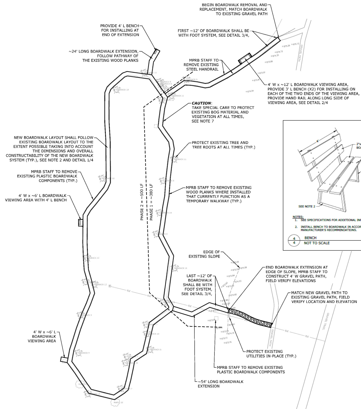
Theodore Wirth Quaking Bog Boardwalk Plans and Details
