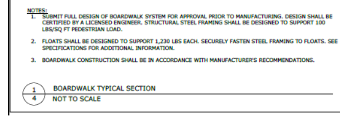
Theodore Wirth Quaking Bog Boardwalk Plans and Details
