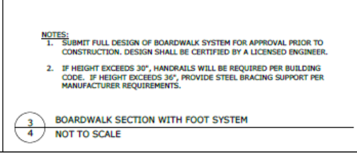
Theodore Wirth Quaking Bog Boardwalk Plans and Details
