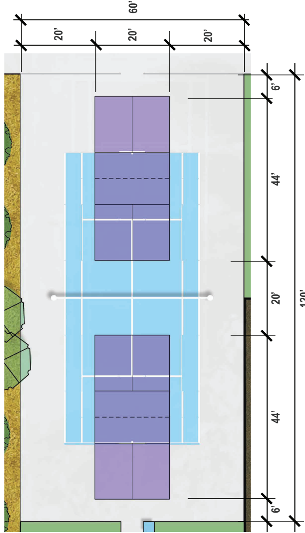
Standard Tennis Court with Pickleball Court Striping Overlay
